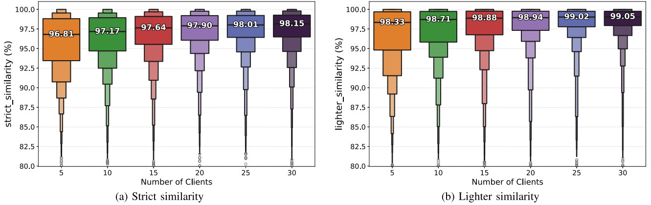
Fig. 4. The similarity score distribution per client across all datasets using boxen plots.
