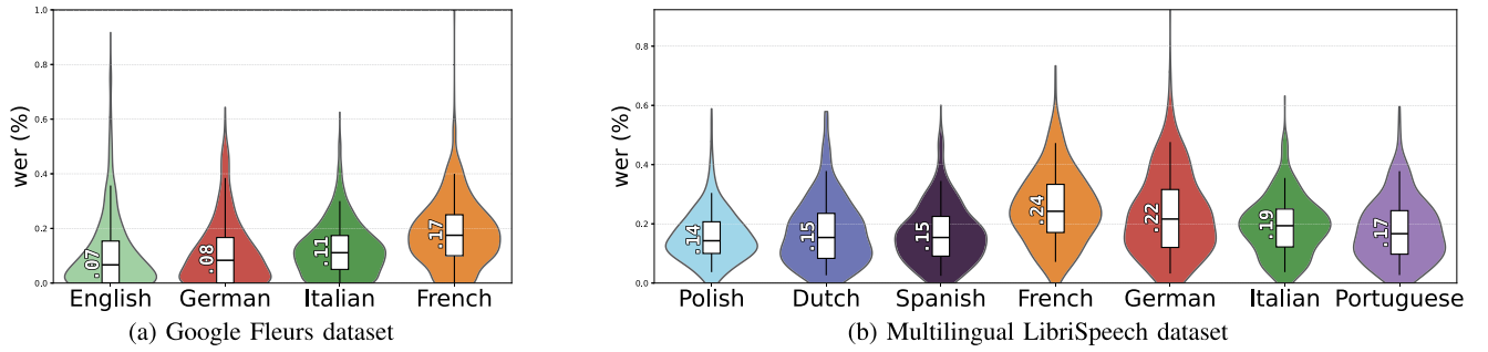
Fig. 6. WER per language across the Multilingual LibriSpeech dataset and Google Fleurs dataset using violin plots.
