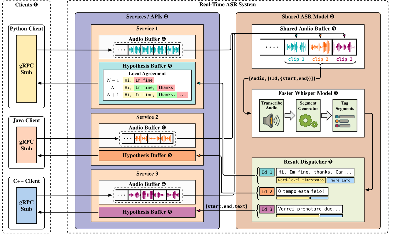
Fig. 1. SWIM architecture. Multiple clients ① stream audio to dedicated services ②, which forward it to a shared ASR model ③ for parallel processing.
