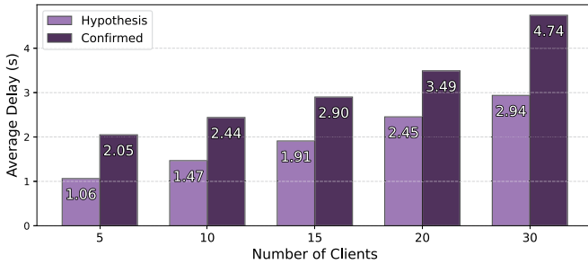
Fig. 7. Hypothesis delay vs Confirmation delay with fixed chunk duration of 1.0 s on Multilingual LibriSpeech dataset.
