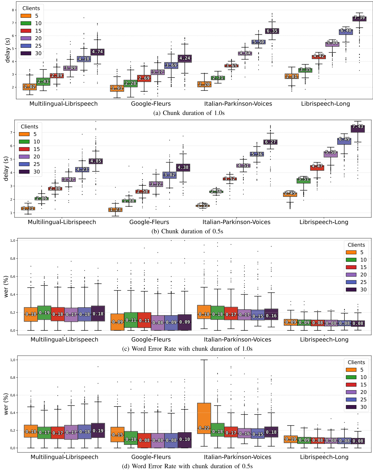
Fig. 3. Evaluation results with different chunk durations using box plots.
