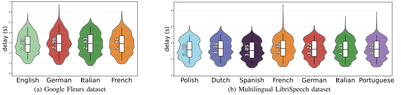
Fig. 5. Delay per language across the Multilingual LibriSpeech dataset and Google Fleurs dataset using violin plots.
