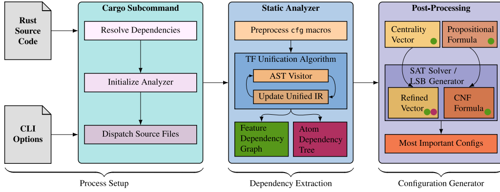
Figure 1. The phases of RustyEx (inspired from Li et al. (2021)).
