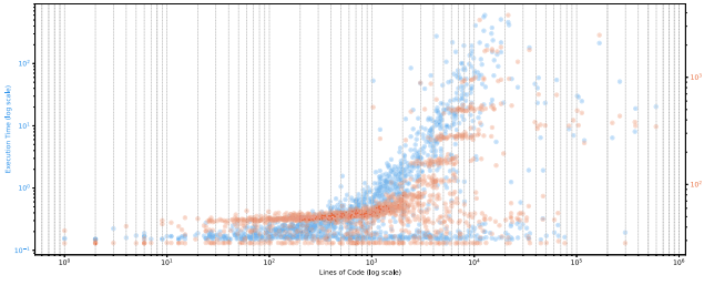
Figure 3. Correlation between lines of code (x-axis), execution time (s) ●, and peak memory usage (MB) ●.
