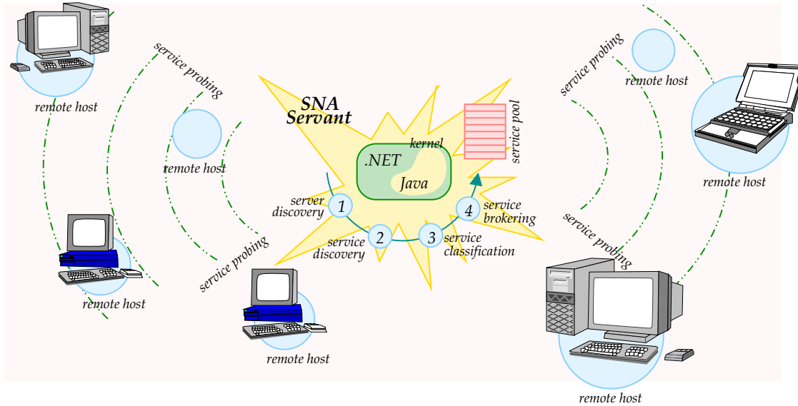
Figure 1. The architecture of the SNA servants and their interaction with the environment.
