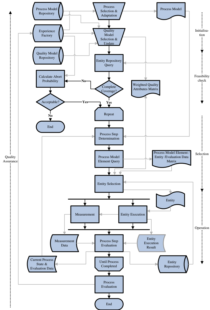
Figure 1. QuaD 2 -Framework [1].
